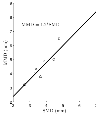
Figure 12. Median Mass Diameter (MMD) as a function of Sauter Mean Diameter (SMD), for the same experimental conditions as in FIG. 10
